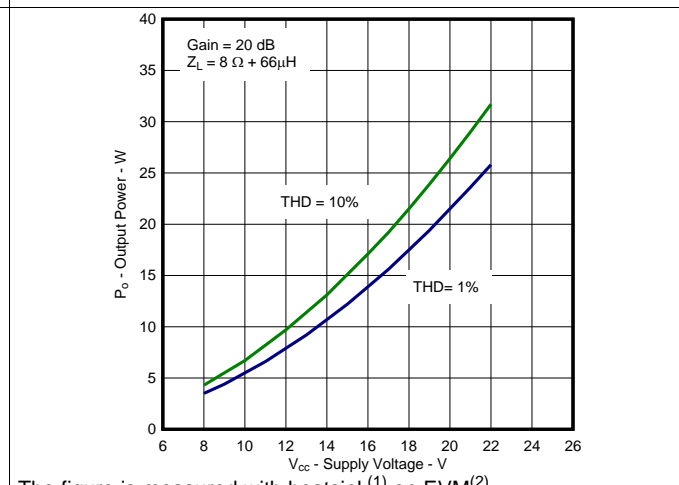
Figure 16. Output Power vs Supply Voltage (BTL)
